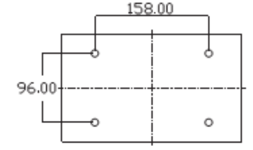
Wall Mounting Hole Dim.
